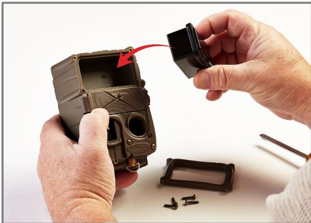
STEP 3: Carefully replace with the required flash module (NB - make sure to line the flash pins up correctly)
