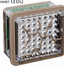
2115 - Power House IR Flash LED module (56 x 850nm High Power LEDs)
